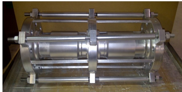
Type 311 dual expansion joint shown with 1" thick, 150# tie rod flanges.
